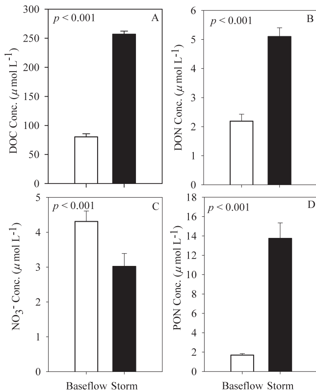
Fig. 2. Average ( \pm SE) concentrations of (A) DOC, (B) DON, (C) \text{NO}_3^- , and (D) PON in the Wailuku River, Hawai'i Island, Hawai'i, during base- and stormflow conditions. Data from the two sites were combined because there were no significant differences in concentrations between sites. p values indicate results from two-way ANOVAs and Mann–Whitney U -tests for flow conditions.
