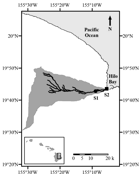
Fig. 1. Map of sites (Site 1 = S1; Site 2 = S2) along the Wailuku River, Hawai'i Island, Hawai'i. Watershed area for the Wailuku River is delineated in gray.
