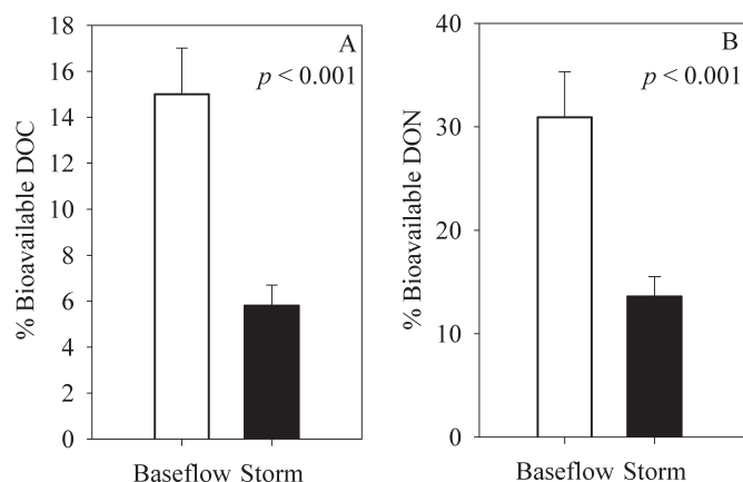
Fig. 3. Average ( \pm SE) percentage (A) DOC and (B) DON bioavailability in the Wailuku River, Hawai'i Island, Hawai'i, during base- and stormflow conditions. Data from the two sites were combined because there were no significant differences in DOM bioavailability between sites. p values indicate results from two-way ANOVAs for flow conditions.
