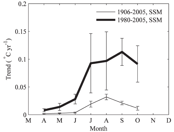
Fig. 6. Rates of warming as a function of month from the SSM site. Light line: 1906–2005. Heavy line: 1980–2005 (similar to the analysis of [Austin and Colman 2007]).
