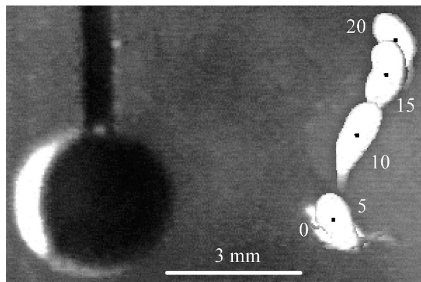
Fig. 2. Escape to the pounce-mimic stimulus showing superimposed images of a copepod ( Tortanus discaudatus ) at 5-ms intervals following the abrupt movement of the 3-mm cylindrical bar seen on the left. Note the initial reorientation upward, followed by acceleration (during pereopod power stroke) and deceleration (after completion of power stroke and during return stroke) in this single-“kick” escape. Pereiopods cannot be seen in this sequence. Black square on the image of the animal indicates center of gravity, which was used to determine the escape trajectory. The peak cylinder velocity used to trigger this escape was 8.8 \text{ cm s}^{-1} , which computes to a movement of \sim 4 \text{ cm s}^{-1} of the animal or a water deformation rate of 17 \text{ s}^{-1} .
