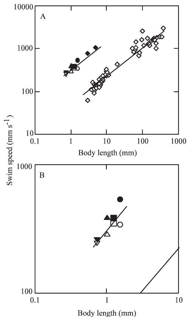
Fig. 9. (A) Maximum swim velocities scaled by organism length in response to the bar (closed symbols) and suction (open symbols) stimuli. Circles: Tortanus discaudatus ; squares: Centropages hamatus ; triangles: Acartia hudsonica ; inverted triangles: Temora longicornis . Other symbols: open diamond: fishes (Domenici and Blake 1997; Shepherd et al. 2000; Williams et al. 1996); closed diamond: calanoid copepods (Lenz et al. 2004). Both solid lines indicate slope: L^{2/3} . (B) Maximum swim velocities measured in current experiment. Symbols are the same as in panel (A). Lines indicate slopes of L^{2/3} drawn on the left for copepod and on the right for fish data.
