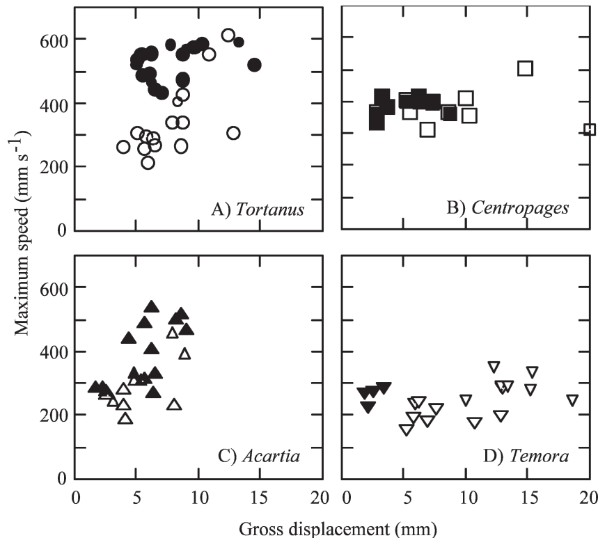
Fig. 7. Gross displacement vs. maximum escape speeds for the two stimuli (bar: closed symbols; suction: open symbols) and four species: (A) Tortanus discaudatus ; (B) Centropages hamatus ; (C) Acartia hudsonica ; and (D) Temora longicornis . Smaller symbols indicate displacements produced by individuals that swam offscreen.
