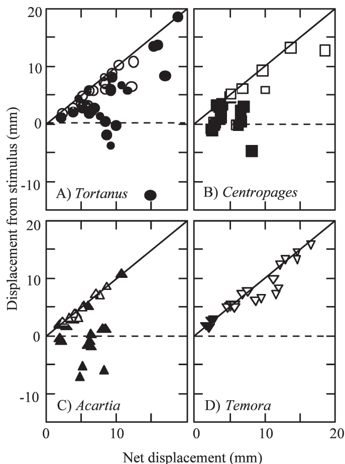
Fig. 8. Efficiency of escape trajectory: increase in distance from stimulus (y-axis) vs. net displacement from starting point (x-axis). Forty-five degree slope indicates escape trajectories directly away from stimulus and thus represents an efficiency of 100%. The dashed horizontal line indicates that the escape did not increase the distance between the organism and the stimulus. Points represent data for individual escapes (bar: closed symbols; suction: open symbols), and four species: (A) Tortanus discaudatus ; (B) Centropages hamatus ; (C) Acartia hudsonica ; and (D) Temora longicornis . Smaller symbols indicate displacements produced by individuals that swam offscreen.
