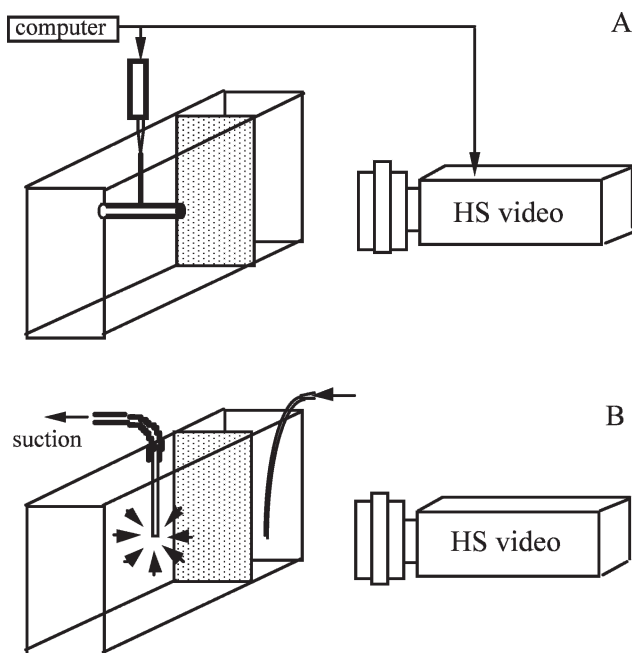
Fig. 1. Diagram of stimulus and filming setups. (A) Bar stimulus: escape responses were generated by rapid movements of a plastic cylinder under computer control. (B) Suction stimulus: escapes were produced when the copepod was drawn sufficiently close to the orifice of a suction tube. A mesh window divided the chamber into two compartments. A cotton filter was fitted into the right compartment for the suction stimulus. Arrows indicate direction of water flow.
