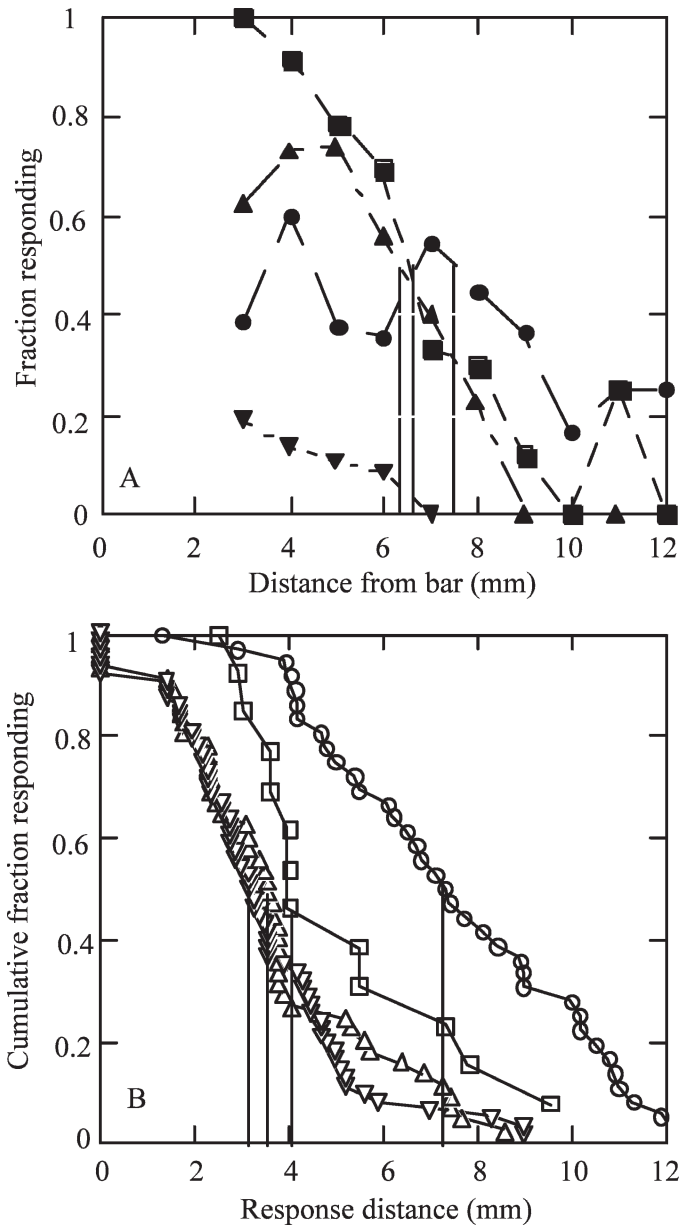
Fig. 4. Probability of an escape response as a function of distance from stimulus. (A) Bar stimulus: points plotted are the fraction of the number of individuals of a given species producing escapes to the total number of individuals at the same distance from the center of the cylinder (1-mm bins). (B) Suction stimulus: ordinate of each point is the cumulative fraction of escapes triggered at the distance given by the abscissa; points at x = 0 represent animals "captured" by the suction tube. Vertical lines indicate the 50% escape distance for each species. Circles: Tortanus discaudatus ; squares: Centropages hamatus ; triangles: Acartia hudsonica ; inverted triangles: Temora longicornis .
