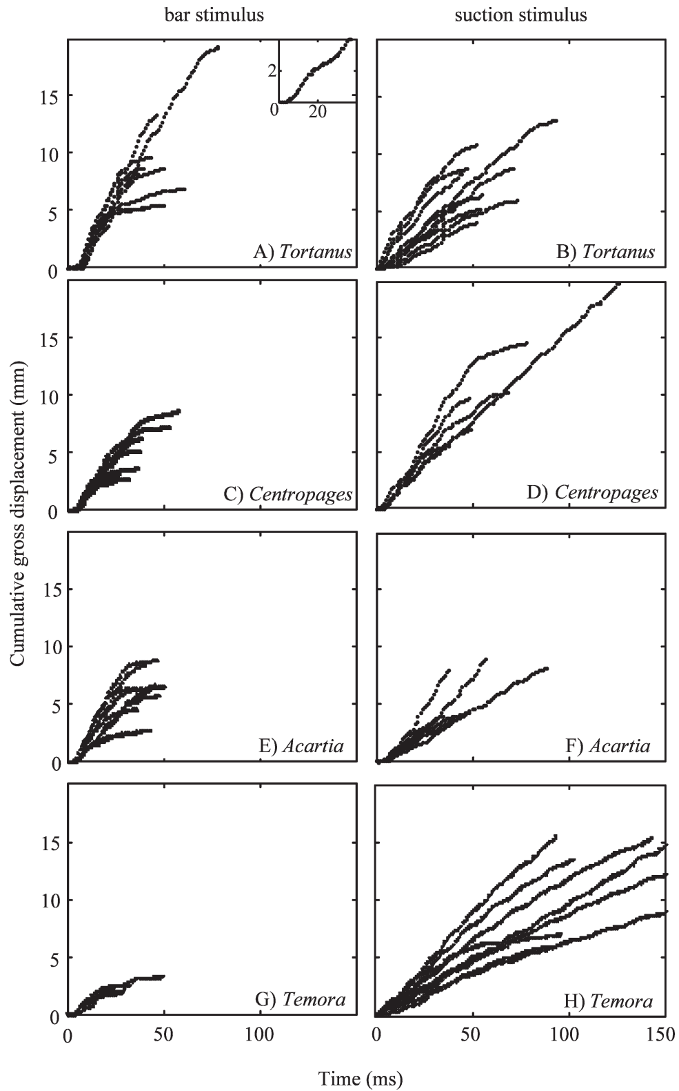
Fig. 6. Gross displacement over time in escape responses to (A,C,E,G) bar stimulus and (B,D,F,H) suction stimulus for the four species. Inset in (A) shows the trajectory for a single escape for the first 40 ms. Gross displacement was measured at 1-ms intervals from the beginning of the stimulus for the bar ( T = 0 ) and first detectable escape movement for the suction.
