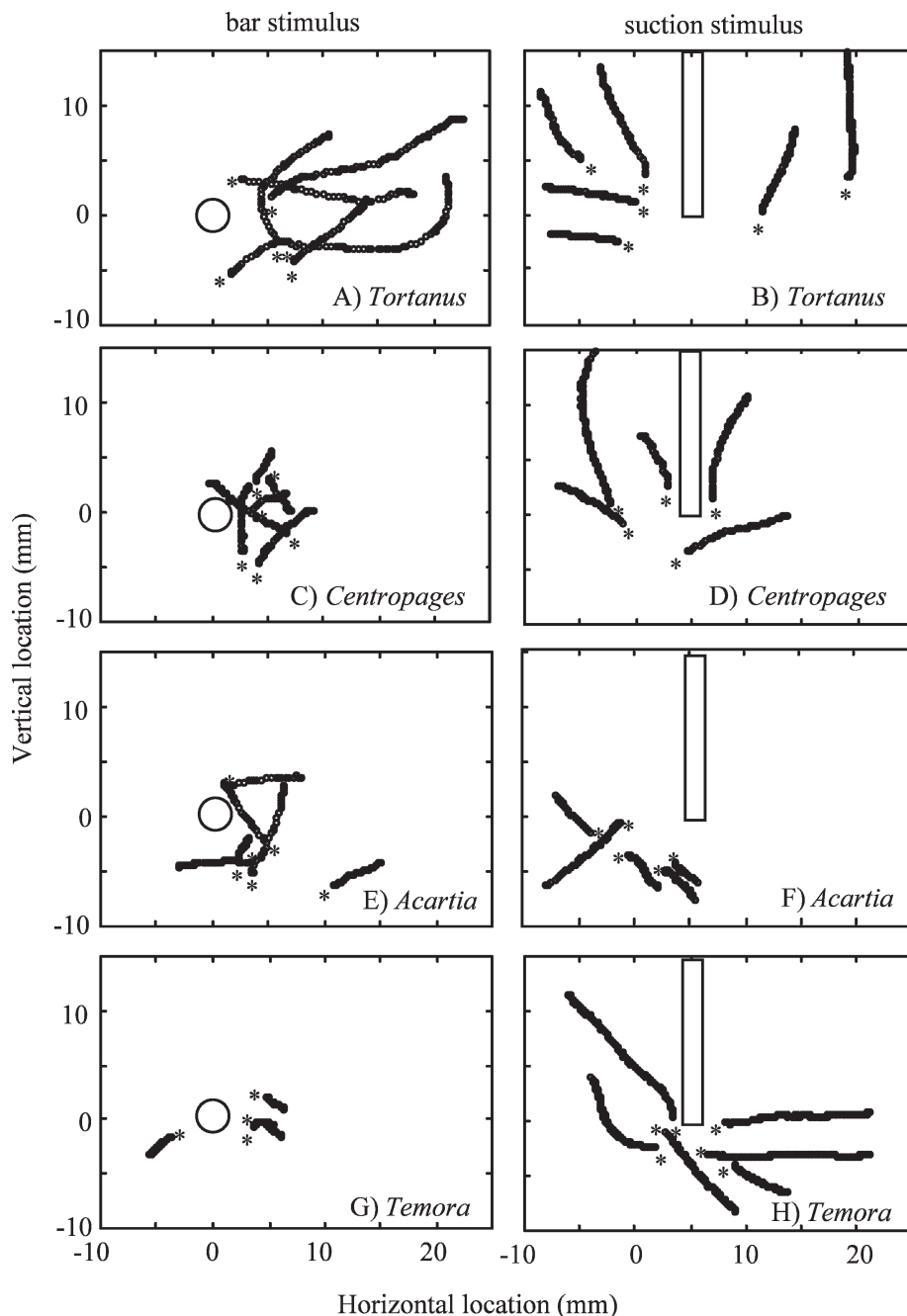
Fig. 3. Escape trajectories for four species of calanoid responding to two hydrodynamic stimuli. (A,C,E,G) Escape trajectories in response to an abrupt, brief, 34\text{-}\mu\text{m} movement of a cylindrical bar (bar stimulus); bar location is indicated by large open circle. (B,D,F,H) Escape trajectories in response to a suction tube with a flow rate of 0.85\text{ mL s}^{-1} (suction stimulus); location of suction tube is indicated by the open vertical bar. Asterisks (*) indicate the position at time of initiation of the escape.
