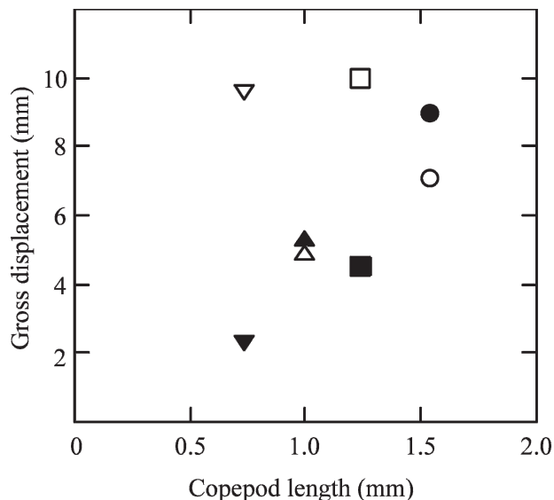
Fig. 10. Copepod length vs. mean escape distances in response to the bar (closed symbols) and suction (open symbols) stimuli. Circles: Tortanus discaudatus ; squares: Centropages hamatus ; triangles: Acartia hudsonica ; inverted triangles: Temora longicornis .
