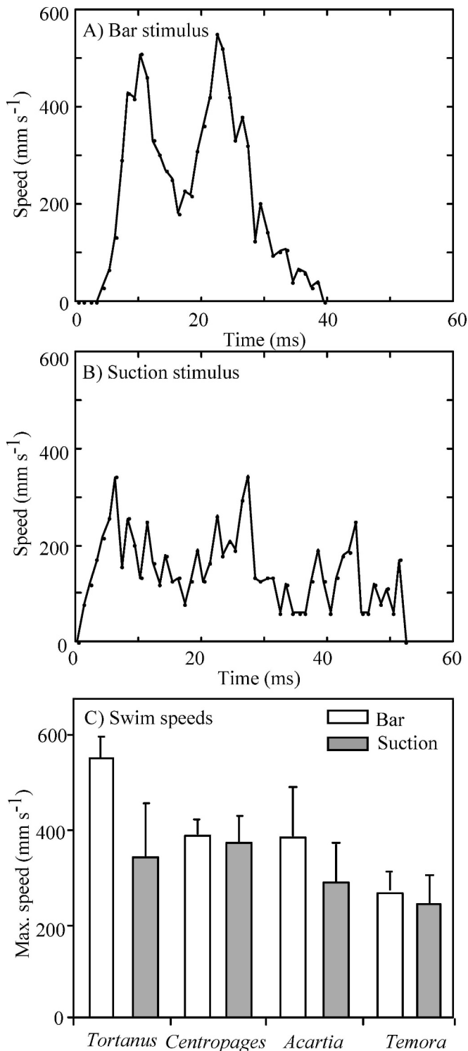
Fig. 5. Swimming speeds for Tortanus discaudatus over time during an escape in response to (A) the bar and (B) the suction stimulus. Swimming speeds were measured at 1-ms intervals. (C) Average maximum swim speeds during escapes from the bar and suction stimulus for four species.
