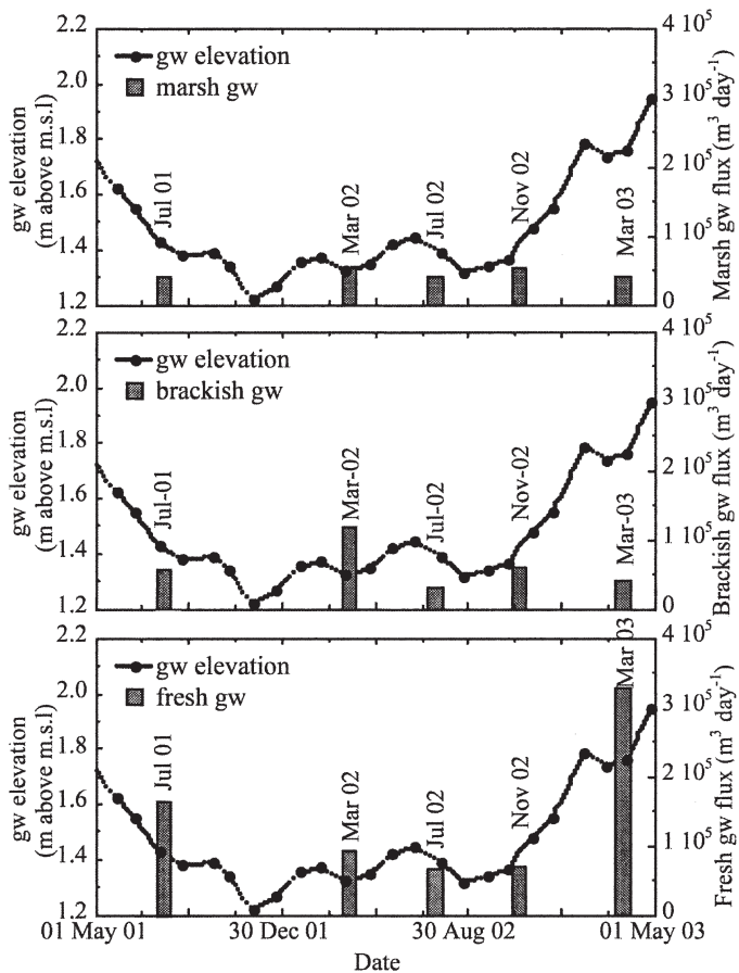
Fig. 9. Marsh, brackish, and fresh groundwater (gw) flux (cubic meters per day) to the Pamet River Estuary for five time periods between July 2001 and March 2003. Also shown is the groundwater elevation (meters above sea level) from a nearby U.S. Geological Survey monitoring well (J561 MA-TSW).
