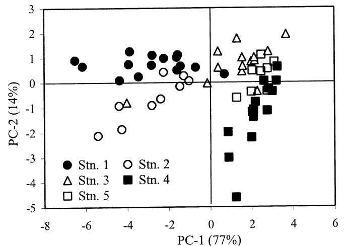
Fig. 5. Euphausia superba . Principal component analysis describing fatty acid profiles of the digestive glands (mg g -1 dry mass). Projection of individuals from different stations on PC1–PC2 plane.
