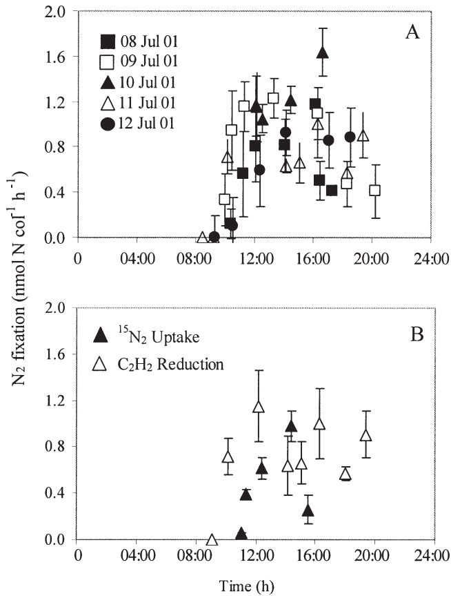
Fig. 2. (A) Rates of gross N_2 fixation (estimated using the C_2H_2 reduction method and a conversion factor of 3) over the course of several days during a cruise on the West Florida shelf in the Gulf of Mexico in July 2001. (B) Paired comparisons of gross N_2 fixation ( C_2H_2 reduction) and net N_2 uptake ( ^{15}N_2 ) rates on 11 July 2001. Error bars are standard deviations from triplicate incubations.
