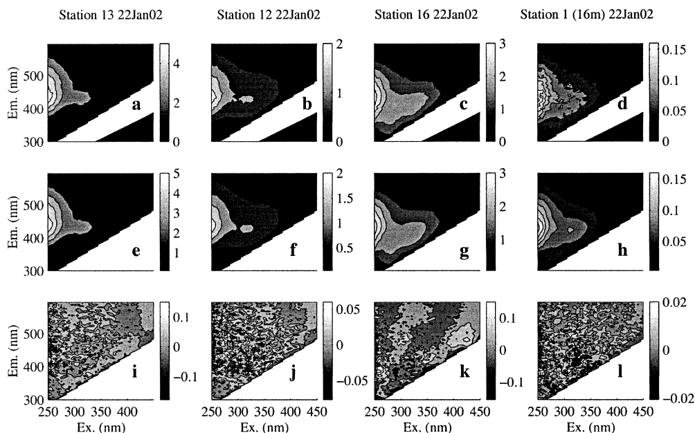
Fig. 2. Examples of (a–d) measured, (e–h) modeled, and (i–l) residual EEMs for four different DOM end members from the catchment. Note the differences in scale between samples and also between the measured and the residual EEMs. Fluorescence is in Raman units.
