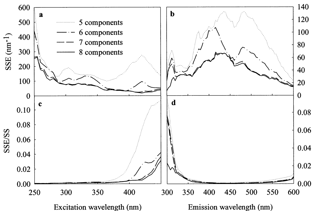
Fig. 4. Analysis of the increase in fit of the model to the measured EEMs with increasing number of components. (a, b) The absolute error as integrated spectra of the sum of squared error (SSE) in the excitation and emission direction, respectively. (c, d) The relative error as the sum of squared error divided by the total sum of squares (SSE/SS). The different lines represent different numbers of components.
