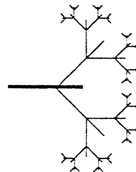
Fig. 8. Branch structure used by Harvey et al. (1995) in flume experiments simulating larval settlement. Multiples of the above two-dimensional structure were assembled to make a three-dimensional branch structure. Branch diameters range from 0.5 to 1.7 mm, with diameter decreasing at each bifurcation.
