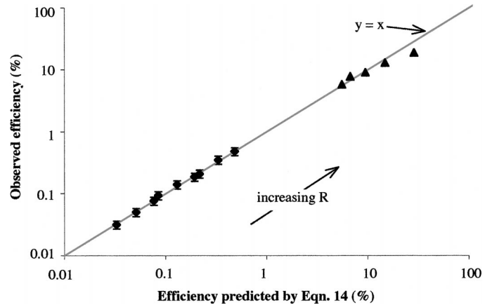
Fig. 7. Comparison of observed capture efficiencies with empirically predicted efficiencies. Observed efficiencies for single-cylinder experiments (black diamonds) are plotted against values predicted by Eq. 14. This empirical relationship also provides good agreement with capture efficiencies on branched structures observed by Harvey et al. (1995) (black triangles).
