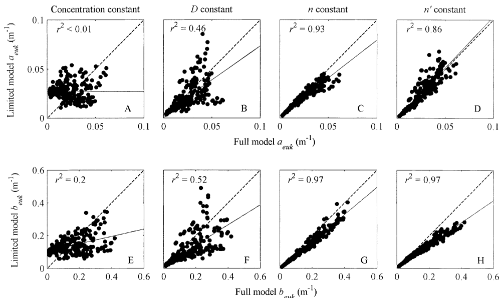
Fig. 7. Sensitivity of (A–D) eukaryotic phytoplankton absorption, a_{\text{euk}} , and (E–H) scattering, b_{\text{euk}} , at 488 nm in the spring to variability in concentration, D , n (488 nm), and n' (488 nm). Full-model values of a_{\text{euk}} and b_{\text{euk}} were calculated using Mie theory and observed values for all four properties (concentration, D , n , and n' ). Limited-model values of a_{\text{euk}} and b_{\text{euk}} were calculated using Mie theory and observed values for three of the properties; the remaining property was held constant at its mean observed value. The effects of variability on b_b were not included because eukaryotic phytoplankton were not important contributors to b_b . The 1:1 line (dashed line) and least-squares regression between full- and limited-model values (solid line) are shown on each plot.
