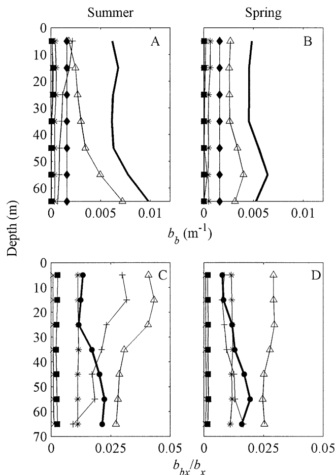
Fig. 6. Depth profiles of constituent contributions to (A, B) backscattering and (C, D) the ratio of constituent backscattering to constituent scattering, b_{bx} : b_x , at 488 nm in the summer and spring. In the term b_{bx} : b_x , x denotes the particle group and “total particle” is the sum of all particle groups. The legend is the same as in Fig. 5.
