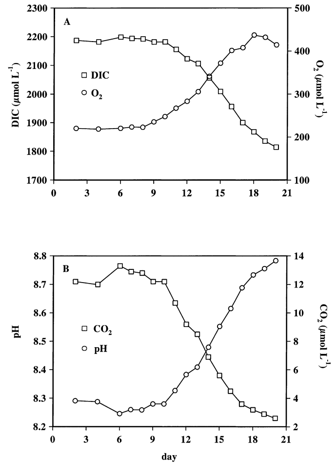
Fig. 4. (A) Inverse development of dissolved inorganic carbon (DIC) and oxygen concentrations in the mesocosm. (B) Draw down of \text{CO}_2 during the phytoplankton bloom and consequent increase in the pH of the water.
