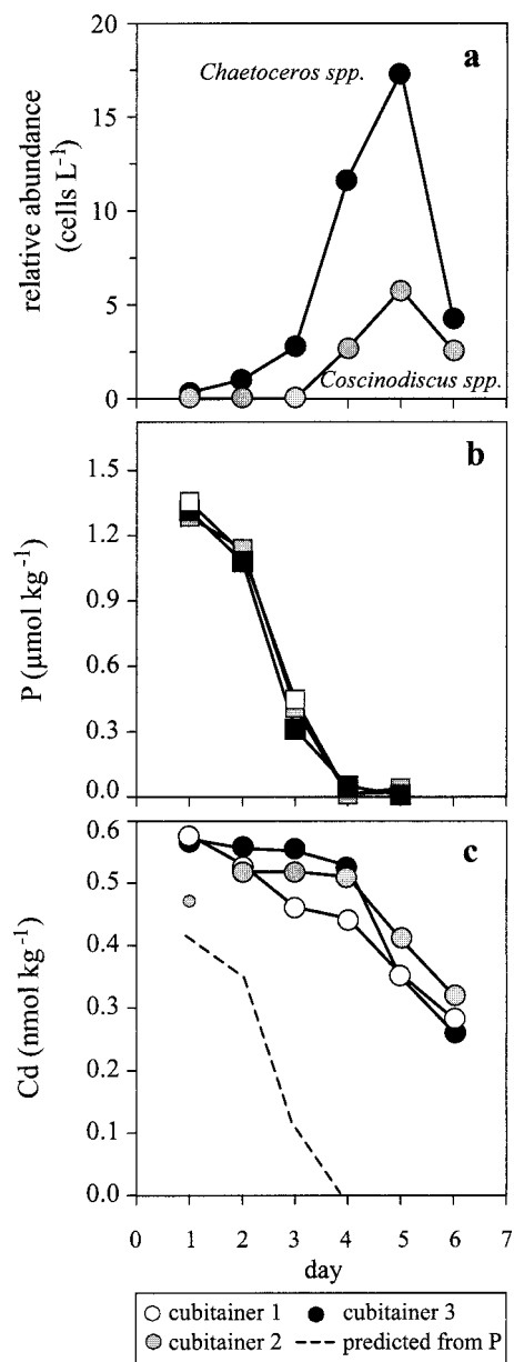
Fig. 5. Changes in (a) relative abundance of Coscinodiscus sp. and Chaetoceros sp. (as counted 5 months after preservation), (b) P, and (c) Cd during a ship-board incubation experiment. Predicted Cd in (c) was found using the Cd/P relation shown in Fig. 3 and measured P. The axes in (b) and (c) have been scaled as in Fig. 4.
